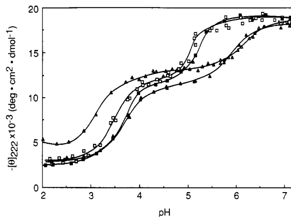
FIGURE 3: Acid denaturation of mutant human apoMbs. [\theta]_{222} is plotted as a function of pH for C110A ( \square ), C110S ( \blacksquare ), C110D ( \blacktriangle ), and C110L ( \triangle ). Conditions were the same as in Figure 2 except that no dithiothreitol was added. Lines through the data points were drawn by inspection.
