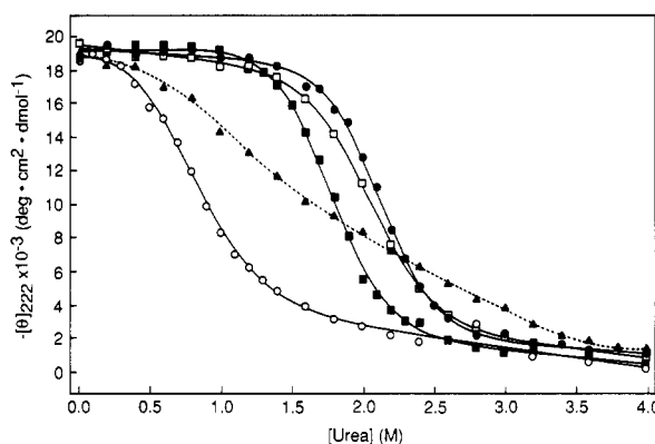
FIGURE 4: Urea denaturation of human apoMbs. [\theta]_{222} is plotted as a function of urea concentration for wild-type ( \square ), C110A ( \bullet ), C110S ( \blacksquare ), C110D ( \circ ), and C110L ( \blacktriangle ). Solid lines are derived by nonlinear least-squares fitting to a two-state transition as described under Experimental Procedures except for C110L, for which the fitting program did not converge. The dashed line was drawn by inspection. Samples were measured at 3 °C and contained, in addition to urea, 1.00 \mu M apoMb and 10 mM HEPES, pH 7.60.
