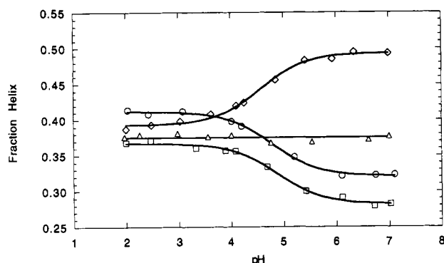
FIGURE 3: Effect of pH on the observed helicity of the Glu peptides at 10 mM NaCl, 0 °C: (◇) E2, (△) E6, (□) E11, and (○) E14. The lines are drawn by inspection only.
